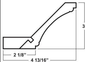
BCWN96 Box Box 48' Beaded Crown
